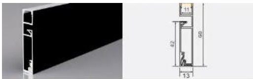
XT818+819 6013 combination skirting L × 60 × 13 mm 10 mm flexible LED strip / rigid LED bar
