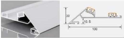
XT-911 10030 floating L × 100 × 30 mm 12 mm flexible LED strip
