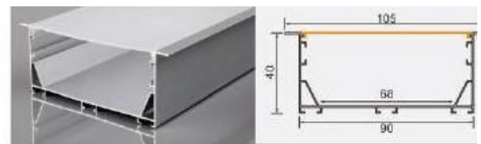
BG-9040A 9040 with flange L × 105 × 40 mm 68 mm flexible LED strip / rigid LED bar
