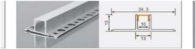
XT757 Single-row perforated 13, double-bottom trim L × 34.3 × 13 mm 10 mm flexible LED strip / rigid LED bar
