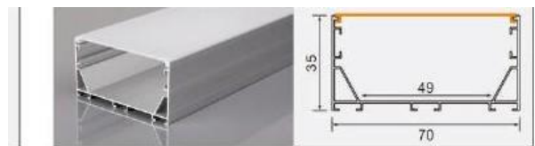
BG-216 7035 L × 70 × 35 mm 49 mm flexible LED strip / rigid LED bar
