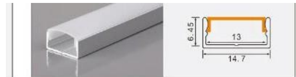
XT506 1507 L × 14.7 × 6.5 mm 13 mm flexible LED strip / rigid LED bar
