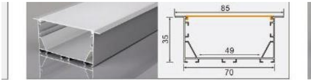
BG-221 7035 with flange L × 85 × 35 mm 49 mm flexible LED strip / rigid LED bar
