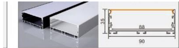
BG157 9035 L × 100 × 35 mm 88 mm flexible LED strip / rigid LED bar
