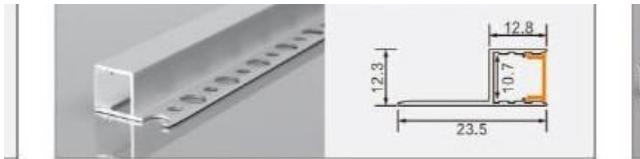
XT759 Single-row perforated 13, side trim L × 23.5 × 12.3 mm 10 mm flexible LED strip
