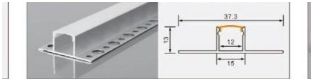
XT732 Single-row perforated 15, double-bottom trim L × 37.3 × 13 mm 12 mm flexible LED strip / rigid LED bar
