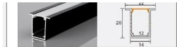
XT581 1420 with flange L × 22 × 14 mm 12 mm flexible LED strip / rigid LED bar
