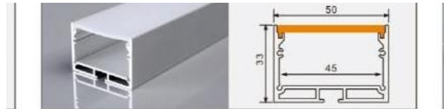
XT413 5033 floor walk-on L × 50 × 33 mm 45 mm flexible LED strip / rigid LED bar
