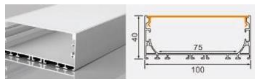
BG05 10040 L × 100 × 40 mm 75 mm flexible LED strip / rigid LED bar
