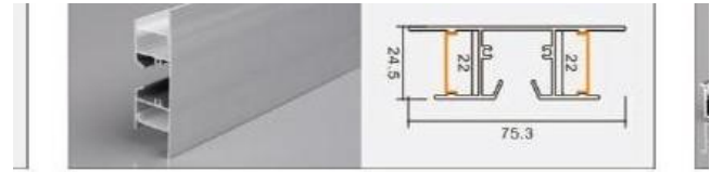
XT572 7525 wall light L × 75.3 × 24.5 mm 22 mm flexible LED strip
