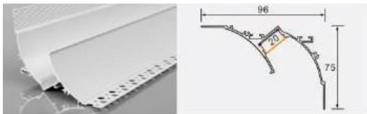
XT801 9675 integrated L × 96 × 75 mm 20 mm flexible LED strip
