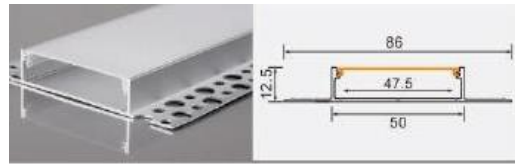
XT1021 5013 double-bottom trim 1.2 L × 86 × 12.5 mm 47 mm flexible LED strip / rigid LED bar
