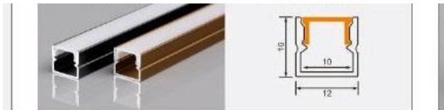
XT537 1210 L × 12 × 10 mm 10 mm flexible LED strip / rigid LED bar
