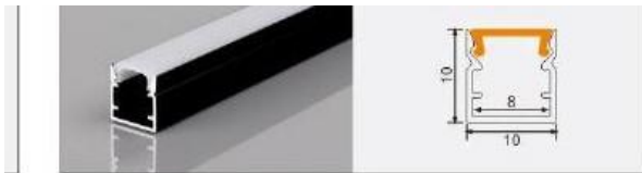
XT453 1010 L × 10 × 10 mm 8 mm flexible LED strip / rigid LED bar
