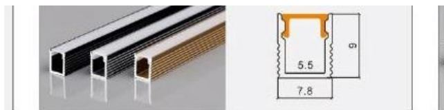
XT231 0809 L × 7.8 × 9 mm 5.5 mm flexible LED strip / rigid LED bar
