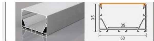
BG-215 6035 L × 60 × 35 mm 39 mm flexible LED strip / rigid LED bar
