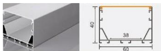
BG-6040M 6040 L × 60 × 40 mm 38 mm flexible LED strip / rigid LED bar
