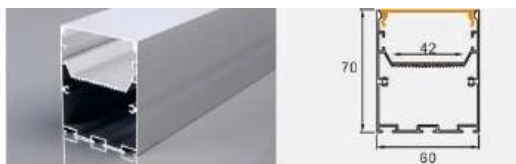
BG96 6070 L × 60 × 70 mm 42 mm flexible LED strip / rigid LED bar
