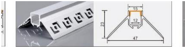
XT679 4723 external-corner trim L × 47 × 23 mm 10 mm flexible LED strip
