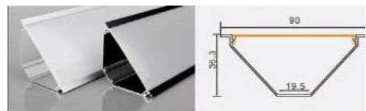
XT587 9036 crown molding L × 90 × 36.3 mm 19 mm flexible LED strip
