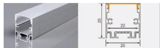
XT372 2525 L × 25 × 25 mm
