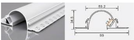
XT787 9935 indirect light L × 99 × 34.5 mm
