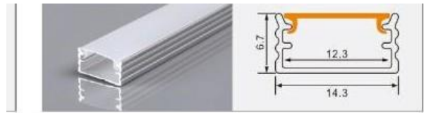
XT45 1407 small flat channel L × 14.3 × 6.7 mm 12 mm flexible LED strip / rigid LED bar
