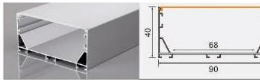
BG-9040M 9040 L × 90 × 40 mm 68 mm flexible LED strip / rigid LED bar
