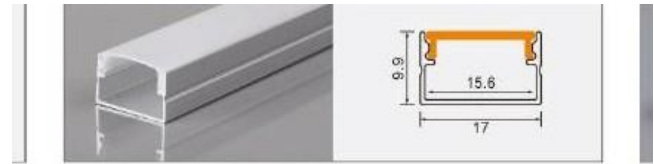
XT950 1710 L × 17 × 9.9 mm 15 mm flexible LED strip / rigid LED bar
