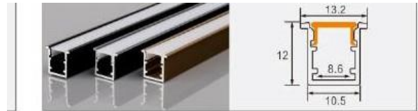
JP22 1112 with flange L × 13.2 × 12 mm 8 mm flexible LED strip
