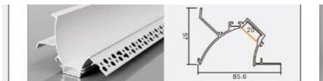
XT693 8657 indirect-light channel, plaster L × 85.6 × 57 mm 20 mm flexible LED strip / rigid LED bar
