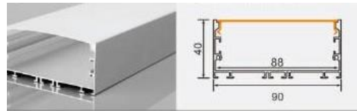
BG51 9040 L × 90 × 40 mm 88 mm flexible LED strip / rigid LED bar
