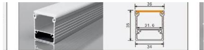
XT412 3435 floor walk-on L × 36 × 35 mm 30 mm flexible LED strip / rigid LED bar
