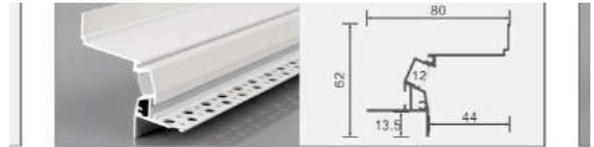
XT-872 8062 L × 80 × 62 mm 12 mm flexible LED strip
