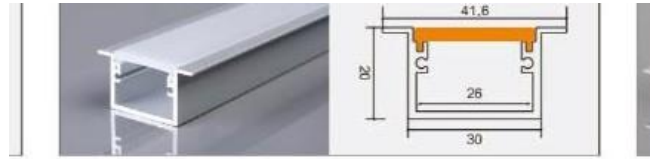
XT558 3020 with flange, floor walk-on L × 41.6 × 20 mm 18 mm flexible LED strip / rigid LED bar
