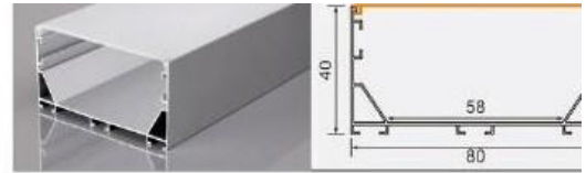
BG-8040M 8040 L × 80 × 40 mm 58 mm flexible LED strip / rigid LED bar
