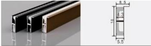
XT471 0618 rear-mount movable — silicone L × 8.5 × 18 mm 5 mm flexible LED strip
