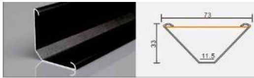
XT642 7333 crown molding L × 73 × 33 mm 11 mm flexible LED strip
