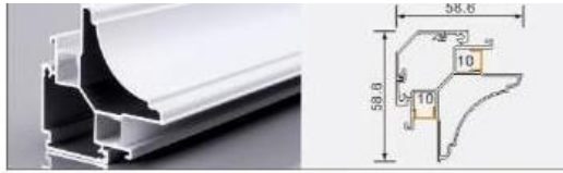
XT835+836 5959 crown molding L × 81.4 × 32 mm 10 mm flexible LED strip
