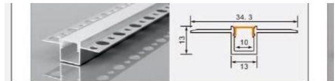
XT758 Single-row perforated 13, double-top trim L × 34.3 × 13 mm 10 mm flexible LED strip / rigid LED bar
