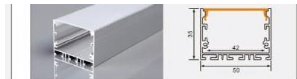
BG63 5035 thick version L × 50 × 35 mm 42 mm flexible LED strip / rigid LED bar
