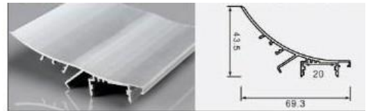
XT564 7044 wall washer L × 69.3 × 43.5 mm 20 mm flexible LED strip / rigid LED bar
