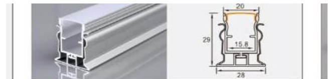
XT511/512 Keel assembly L × 28 × 29 mm 15 mm flexible LED strip / rigid LED bar
