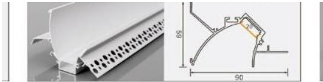
XT573 9059 indirect-light, panel clamp L × 90 × 59 mm 20 mm flexible LED strip / rigid LED bar
