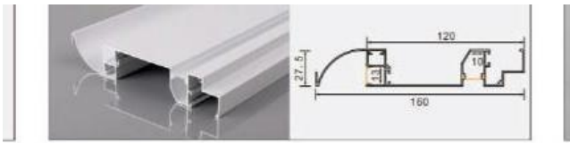
XT988+1005 16027 double-eyelid L × 160 × 27 mm 10 mm flexible LED strip / rigid LED bar
