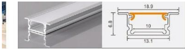
XT993 1307 with flange L × 18.9 × 6.8 mm 10 mm flexible LED strip / rigid LED bar
