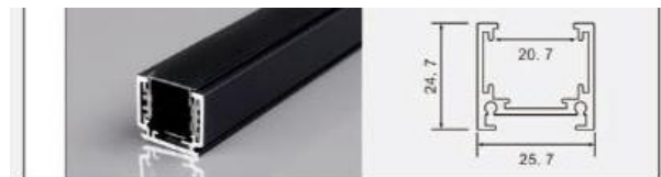
WR-CX-47 Surface-mount L × 25.7 × 24.7 mm 1.6 magnetic-attraction light
