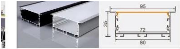
BG70 8035 with flange L × 95 × 35 mm 72 mm flexible LED strip / rigid LED bar
