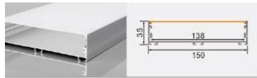
WR15035 15035 L × 150 × 35 mm 138 mm flexible LED strip / rigid LED bar
